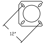
ANCHOR BASE DETAIL 12" BOLT CIRCLE ANCHOR BOLTS: 1" x 36"
