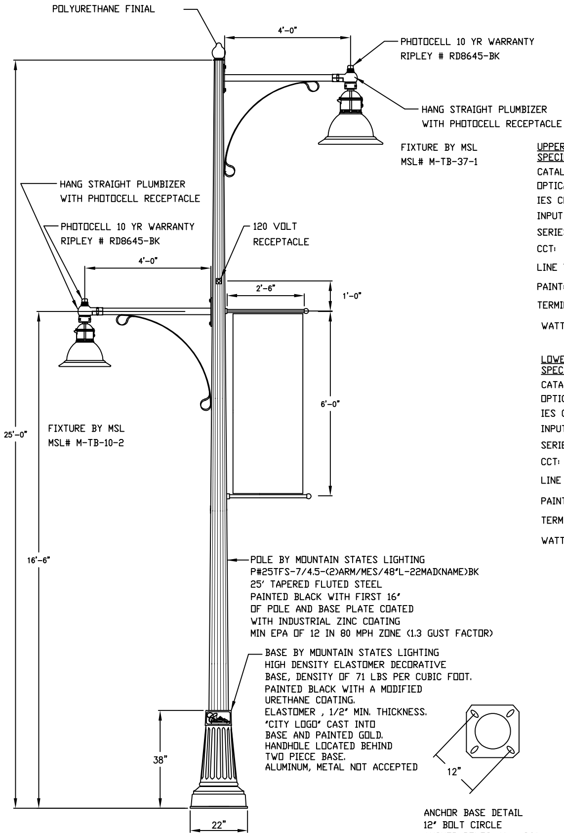
DECORATIVE BASE DETAIL ASSEMBLY COLOR: BLACK
