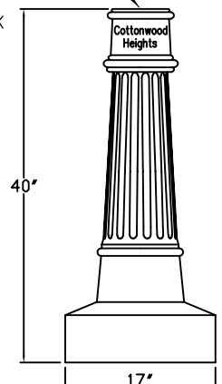
DECORATIVE BASE ENLARGED DETAIL
