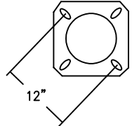
ANCHOR BASE DETAIL 12" BOLT CIRCLE ANCHOR BOLTS: 1" x 36"
